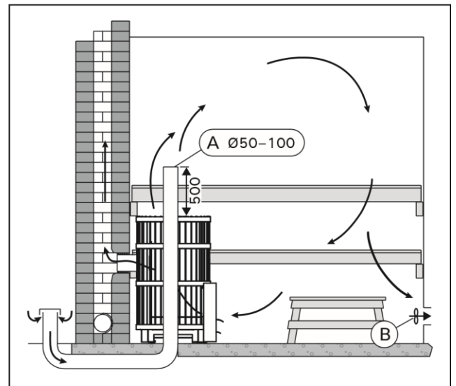
Figure 7. Mechanical exhaust ventilation Abbildung 7. Mechanische Entlüftung similar heat radiation protection.
