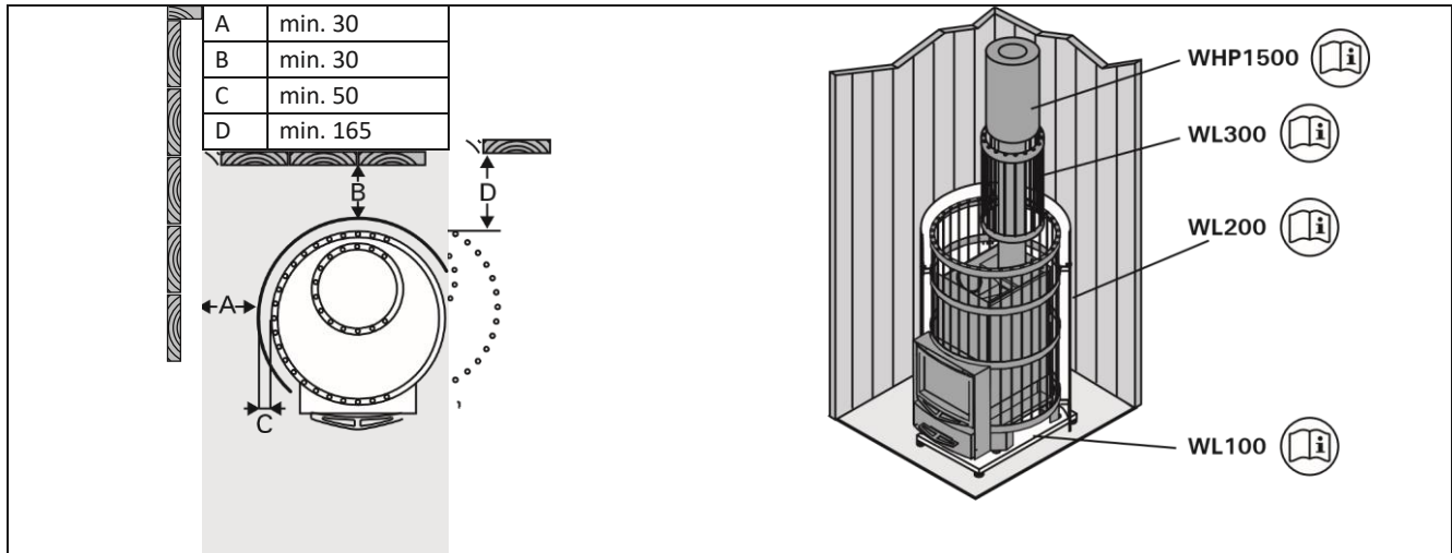
Figure 10. Legend Protection Supplies (all dimensions in millimeters) Abbildung 10. Legend Schutzvorrichtungen (alle Abmessungen in Millimetern)
